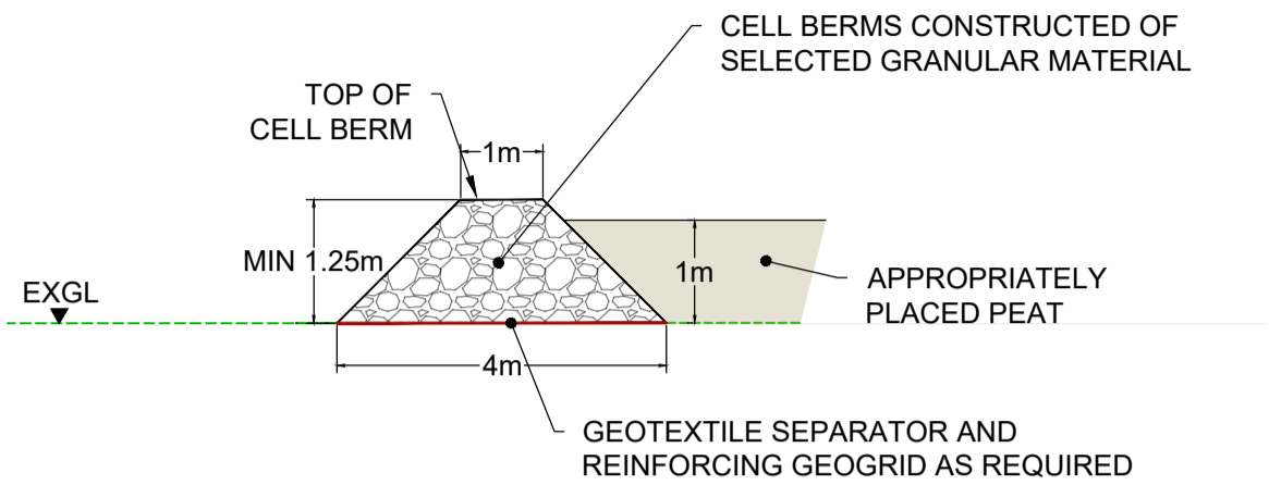
Figure 4-9F Peat Repository PR6 Plan and Section
