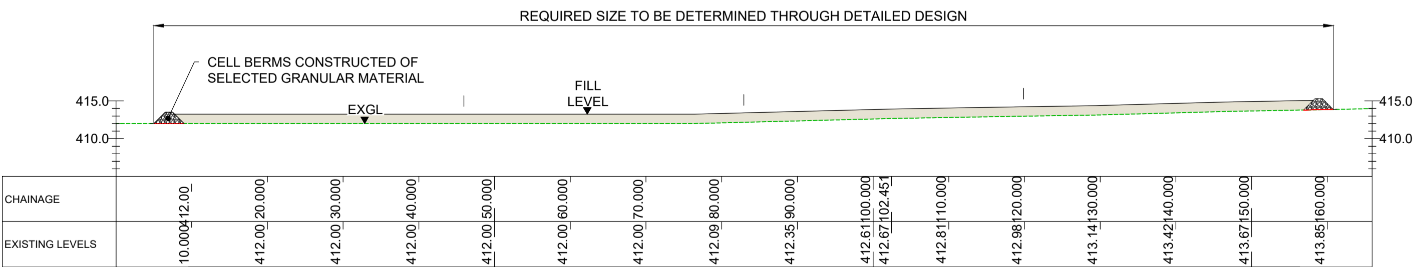
TYPICAL SECTION - PEAT REPOSITORY PR6 SCALE 1:500
