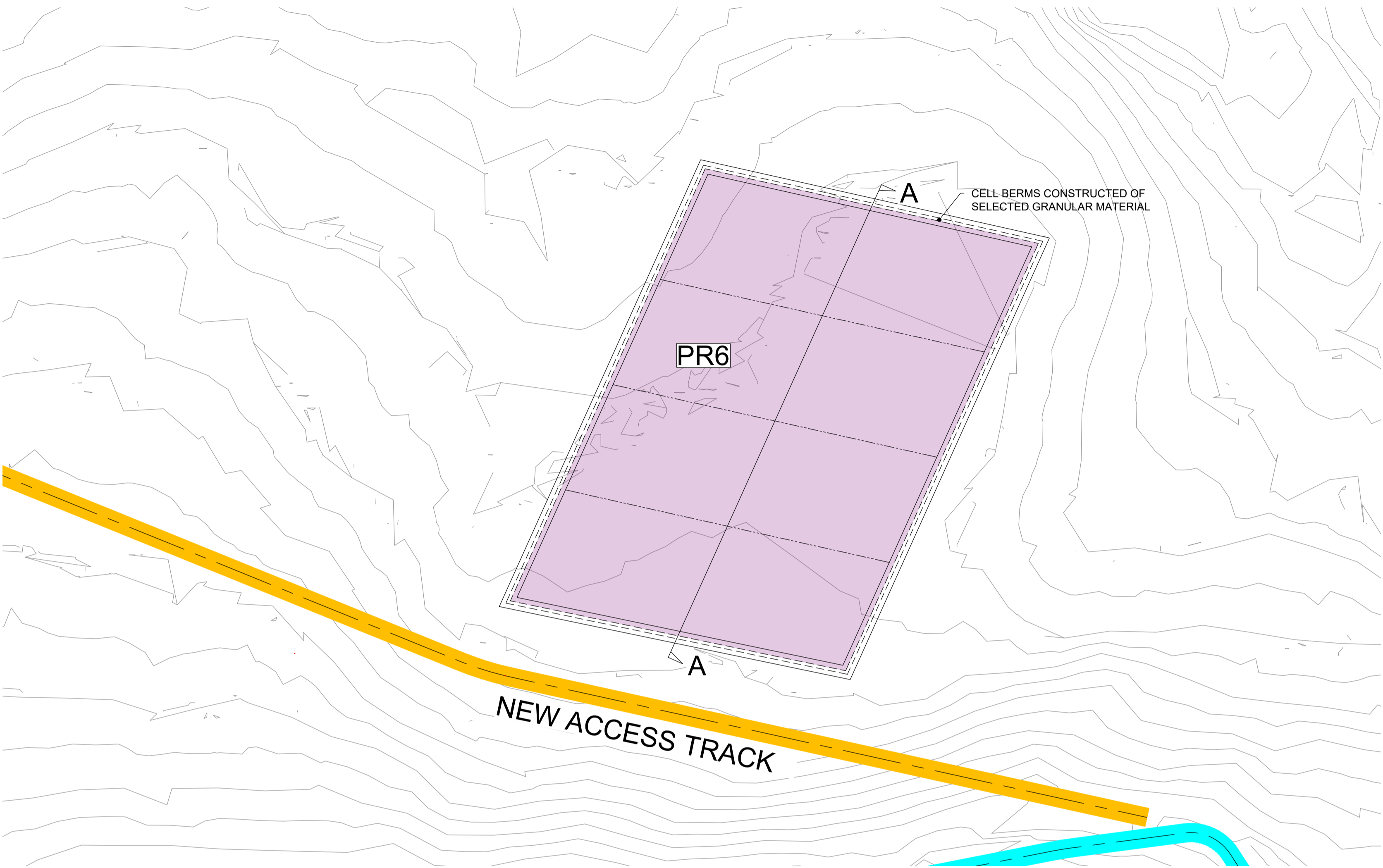
PEAT REPOSITORY PR6 - PLAN VIEW SCALE 1:1000
